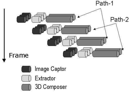
Figure 1: Pipeline Architecture
