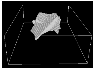
Figure 5: Target Space
